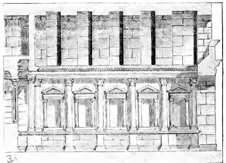
Fig. 493. Nymphæum at Nîmes (restored).
